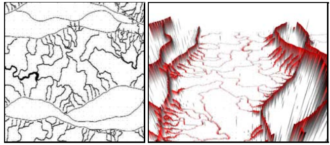
Figure 5: The Midpoint Displacement's Inverse process. The left image shows: in black color the computed elevations and in white color the elevations that still have to be computed. The right image shows the tridimensional view of the D.E.M. : in black/gray color elevations computed with the M.D.I. process (the peaks around the ridges and rivers network (in red)) and in white color the elevations that still have to be computed.
